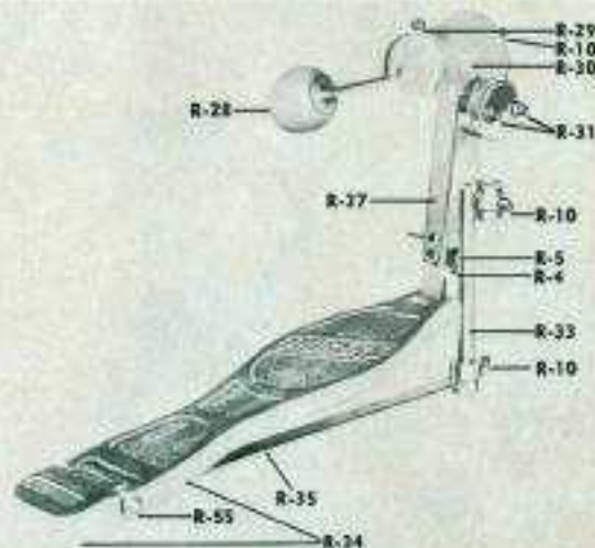
No. 395R "Swivel-omatic" FOOT PEDAL PARTS
