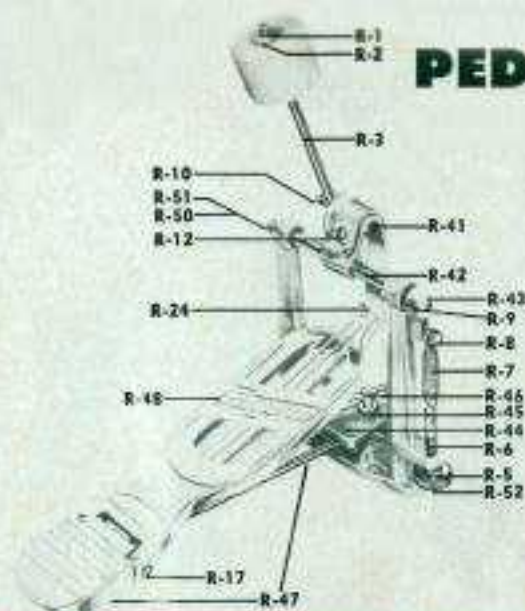
No. 398 "Rocker" FOOT PEDAL PARTS
