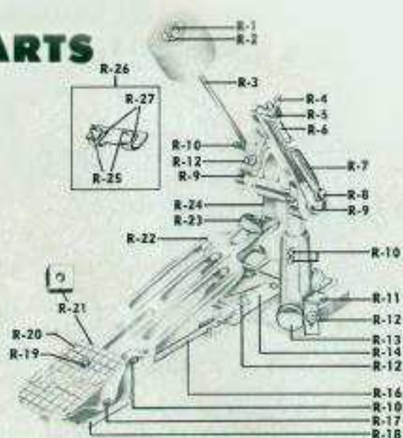
No. 395B "Swivel-omatic" FOOT PEDAL PARTS
