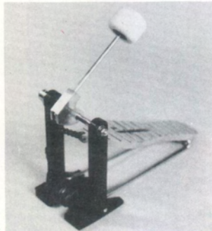
▲ Base Drum Pedal CFP-100 This is the original chain-drive pedal. A sturdy pedal with feather-touch action and never an off-beat squeak. The foot board is engineered to stay at a comfortable angle for both heavy accents and very light beats.
